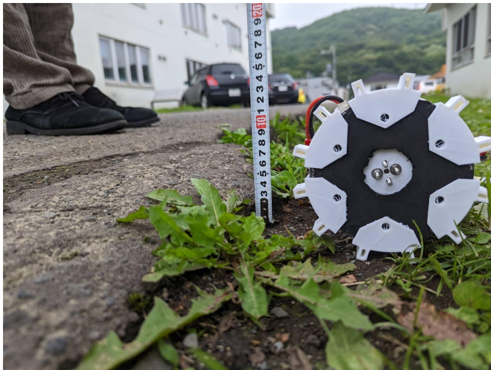
図6.9.2 3～4 [cm] 級段差の横断 (a-2)
